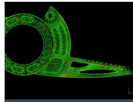
Detailed FE Model
